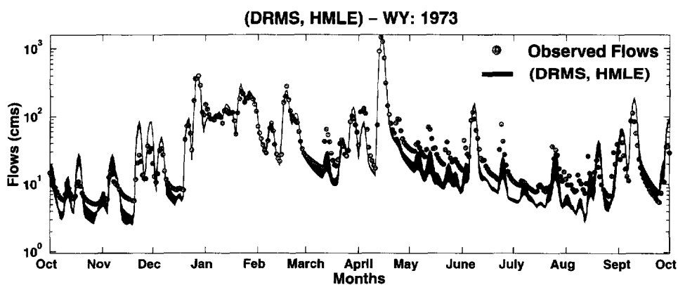
Fig. 8. Hydrograph ranges associated with the Pareto solution set.
